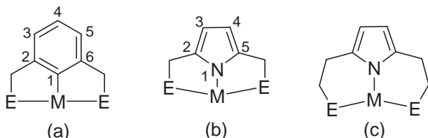
Chart 1. Pincer complexes: E = chelating donor atom.
