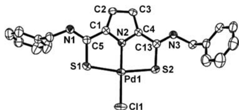
Figure 1. ORTEP view of 2b with thermal ellipsoids drawn at the 50% probability level. Hydrogen atoms and a solvated acetonitrile molecule are omitted for simplicity. Selected bond lengths (Å), angles (°), and torsion angles (°): Pd(1)–Cl(1) = 2.3173(12), Pd(1)–S(1) = 2.3238(10), Pd(1)–S(2) = 2.3256(10), Pd(1)–N(2) = 1.932(3), Cl(1)–Pd(1)–N(2) = 179.16(8), S(1)–Pd(1)–S(2) = 166.78(4), C(2)–C(1)–C(5)–N(1) = 178.8(3), C(2)–C(1)–C(5)–S(1) = 179.4(3).
