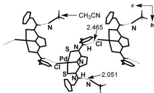
Figure 2. View of 2b from the a axis. The N–H...Cl and N–H...N hydrogen-bonding distances are given in Å.
