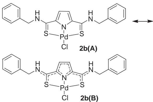
Chart 2. Delocalization of electron in 2b .
